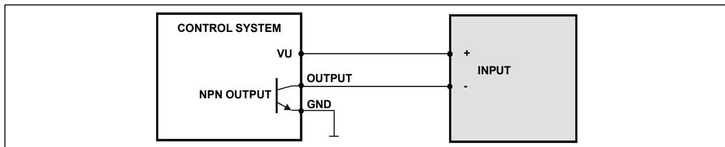
Fig. 2 Connection example with control system with NPN output.
