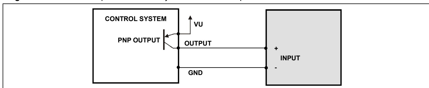
Fig. 3 Connection example with control system with PNP output.
