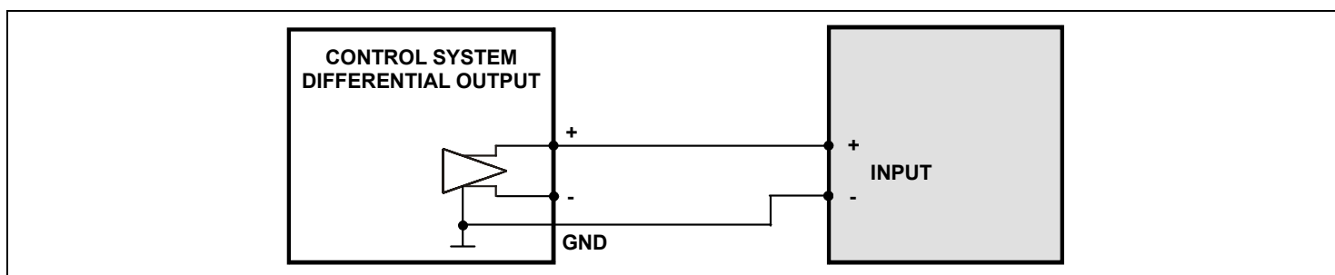
Fig. 5 Connection example with control system with DIFFERENTIAL output (or LINE DRIVER or RS422).
