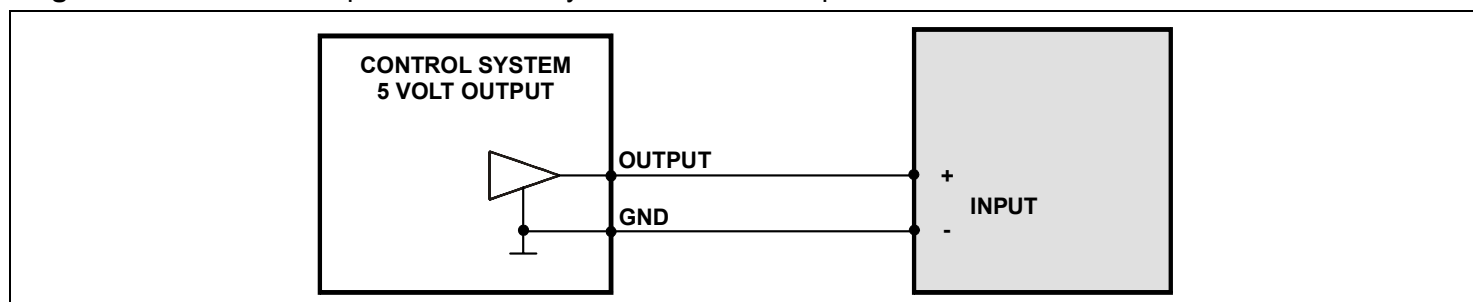
Fig. 4 Connection example with control system with 5 Volt TOTEM-POLE (PUSH-PULL) output.
